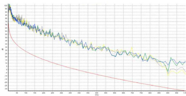
ACR Powersum (dB/100m)
